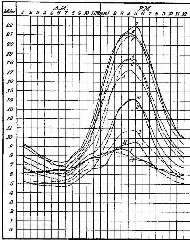
FIG. 6.—Monthly curves of hourly wind velocities.
